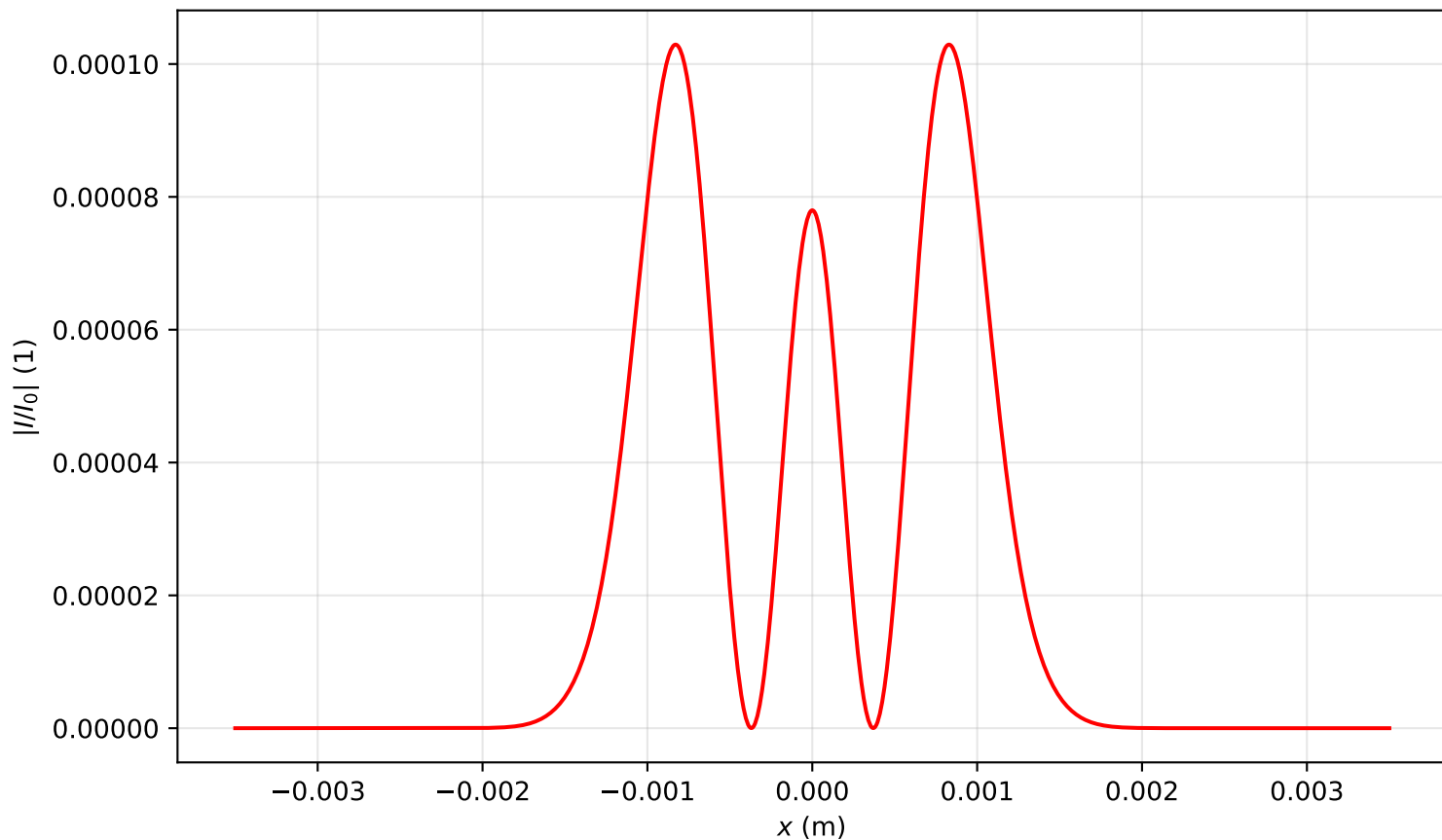
Intensity profile I(x, y = 0, z = 0.637)/I_0 , P_{in}=0.5P_{cr} , artificial time
